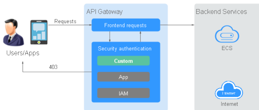
Figure 5-1 Schematic diagram of frontend custom authentication
