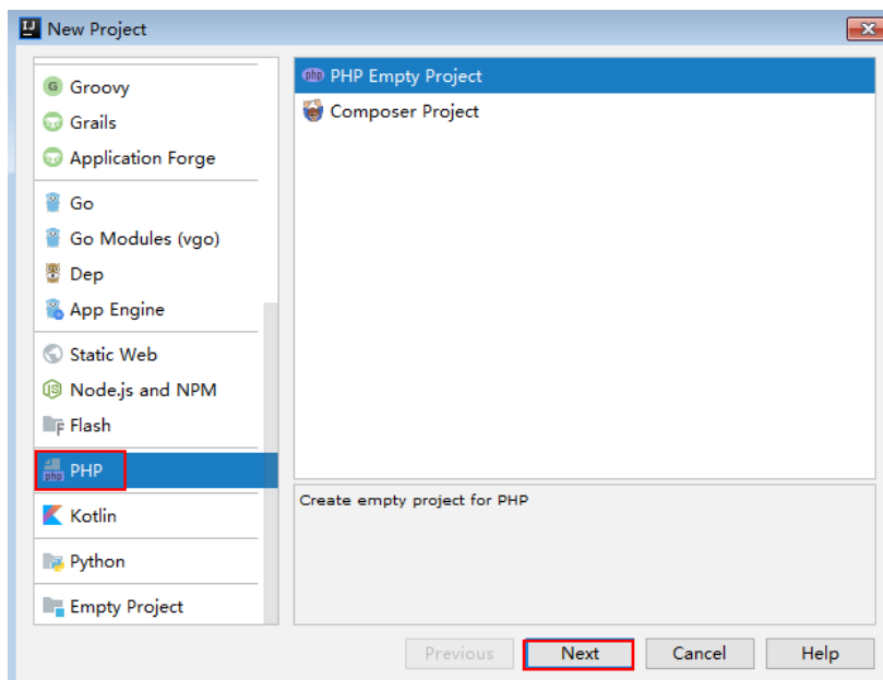
Figure 3-30 PHP
