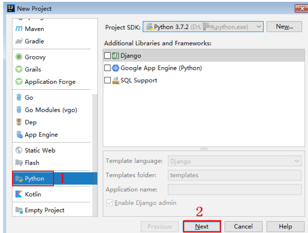
Figure 7-5 New Python
