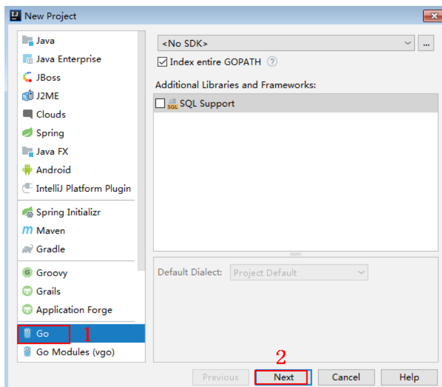
Figure 3-15 Go
