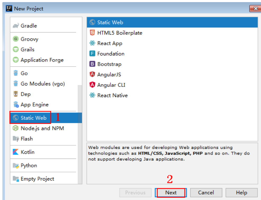
Figure 3-23 Static Web
